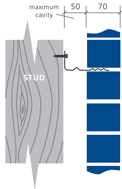
SCREW TIE - SHORT (85MM)
