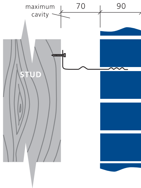
SCREW TIE - LONG (110MM)
